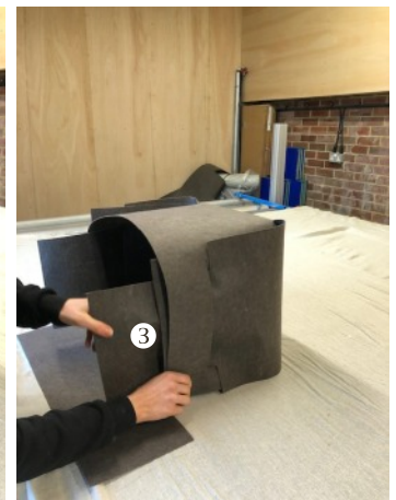
d). Pull post sleeve (3) through slot until edge butts up against slot
